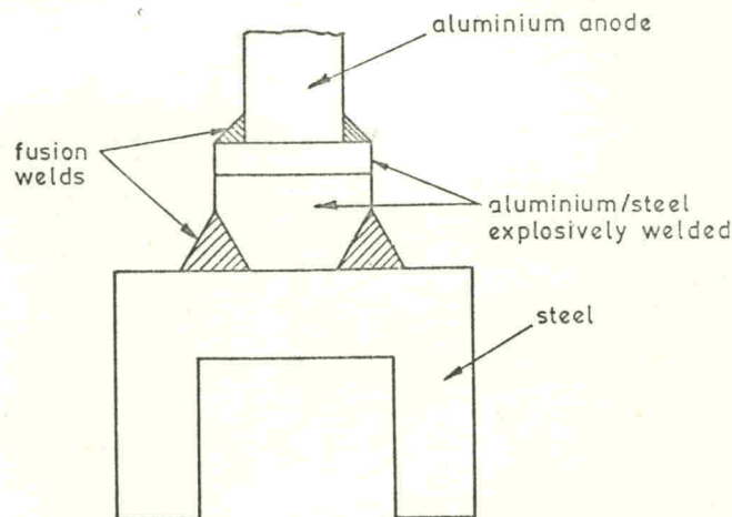
48 Aluminium/steel transition joint. (Stone. 43 )
